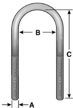
Round Bend
