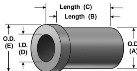
Type 2 - Flat
